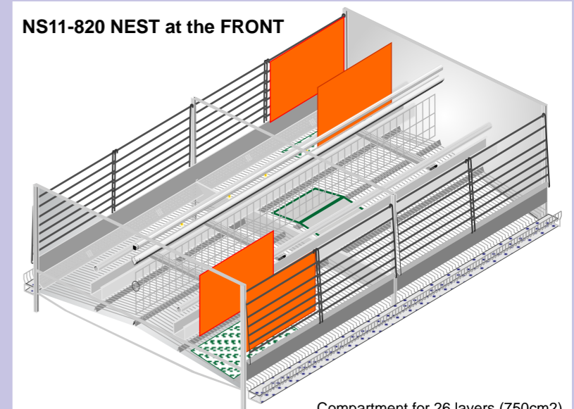
Compartment for 26 layers (750cm 2 )
