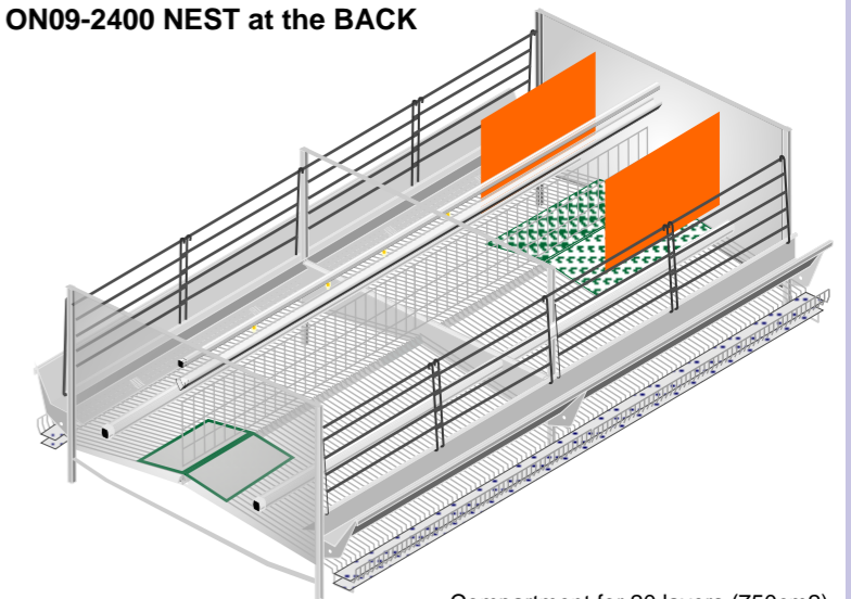
Compartment for 20 layers (750cm 2 )
